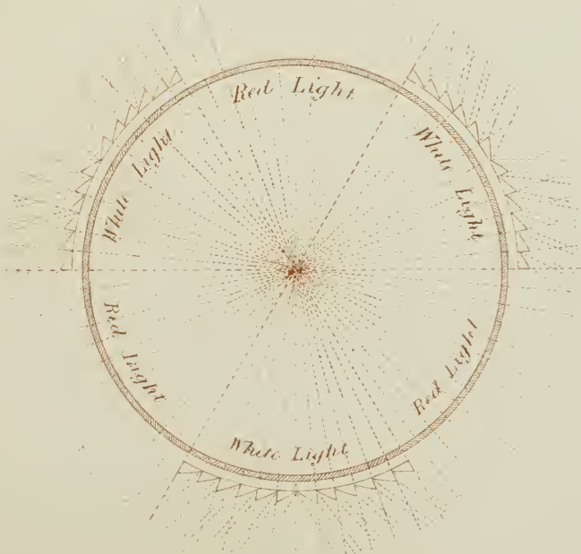
HORIZONTAL FOCAL SECTION showing prisms for Auxiliary Red Light in plan
