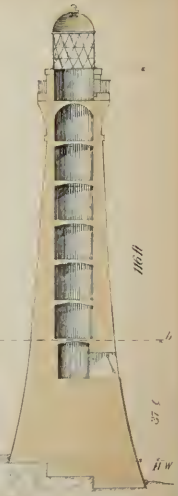
D & T STEVENSON 1869
