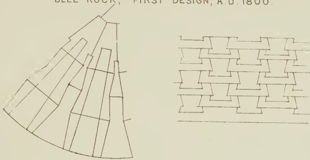
BELL ROCK, FIRST DESIGN, A.D. 1800.
