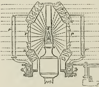
Section. Fig. 41.
