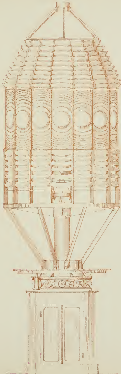
ELEVATION OF THE FIRST DIOPTRIC HOLOPHOTAL REVOLVING LIGHT (1 ST ORDER) DESIGNED OCTOBER 1850, FOR NORTH RONALDSHAY, AND CONTRACTED FOR BY M. LETOURNEAU, ON 3 RD JANU, 1851.
