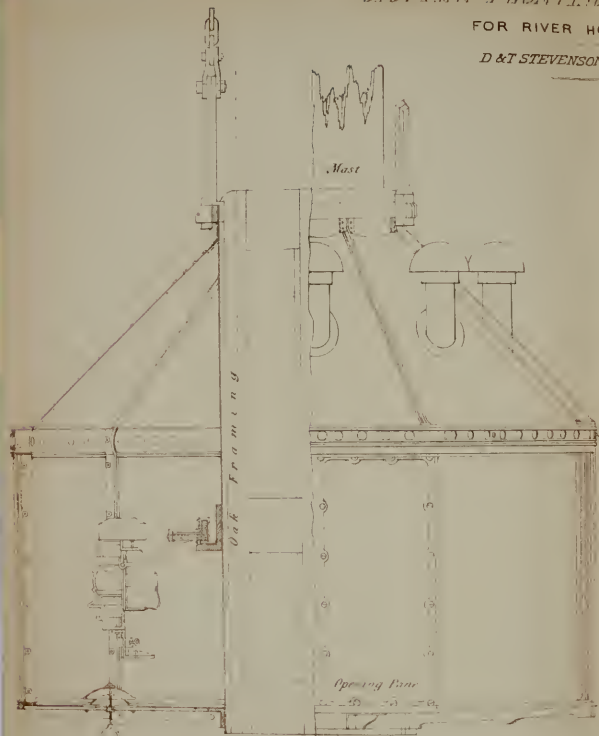
HALF SECTION ON A B
